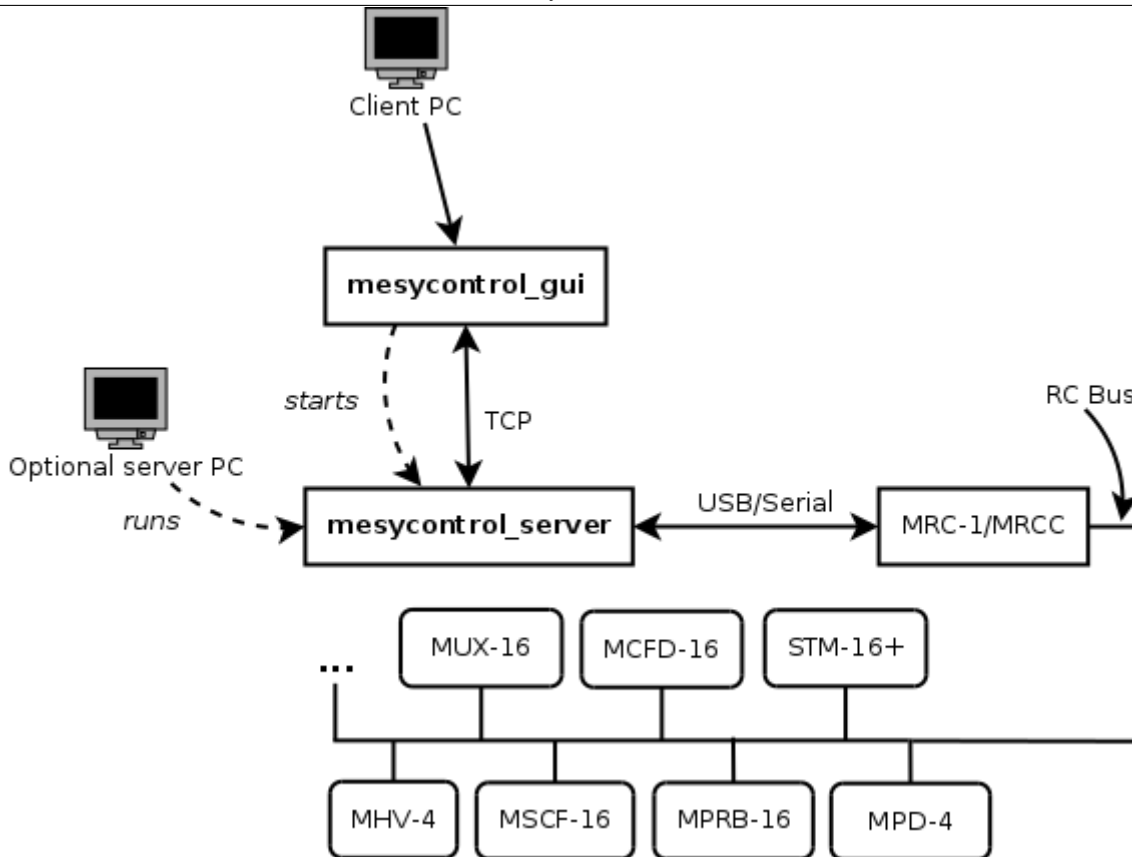
Fig. 1: mesycontrol architecture
